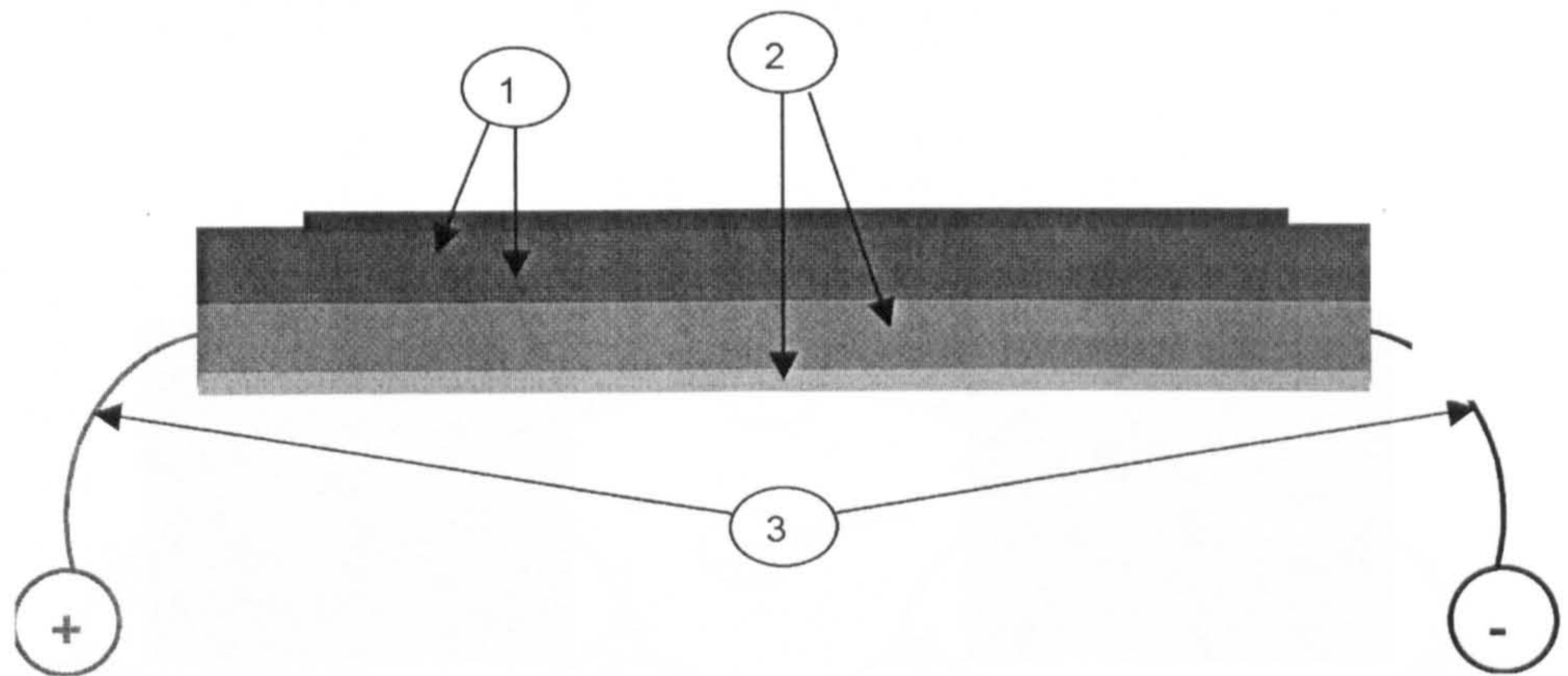
156 (B) A cross section of a basic layered construction used to make colourchange fabric. 1 – textile or other substrate coated with TLCI or TCI, 2 – textile or other substrate coated with conductive ink, which has high resistance, 3 – wires leading to the positive and negative terminals of a power supply.
