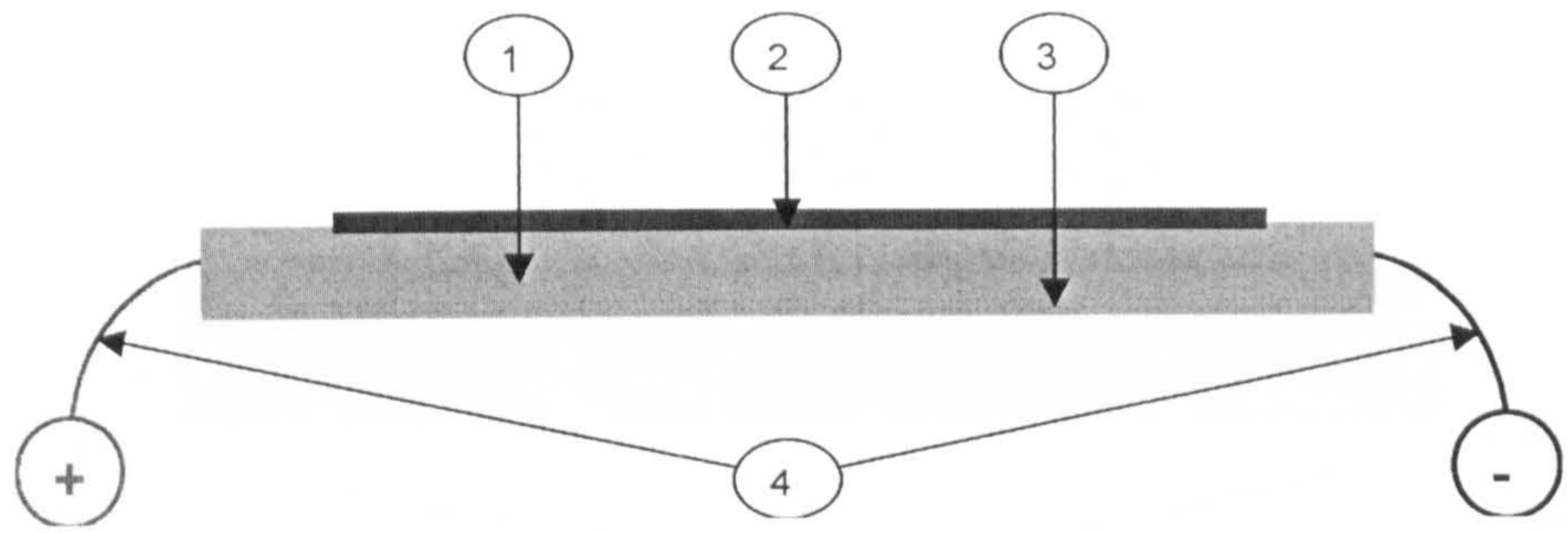
156 (A) A cross section of a basic layered construction used to make colourchange fabric. 1 – textile or other substrate, 2 – TLCI or TCI coating on the substrate, 3 – a layer of conductive ink, which has high resistance on the same substrate, 4 – wires leading to the positive and negative terminals of a power supply.
