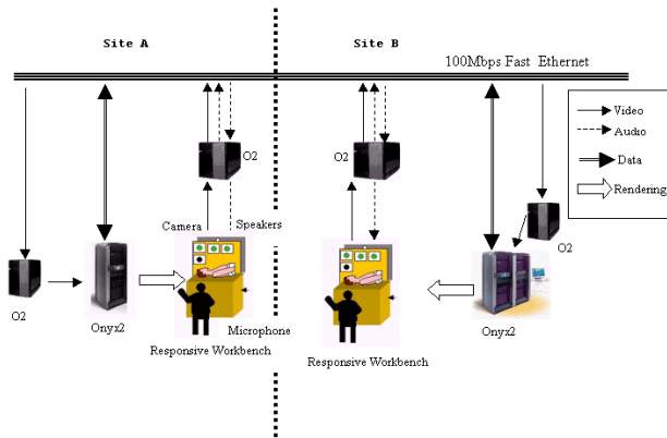
Figure 6: Schematic of the used setup.
