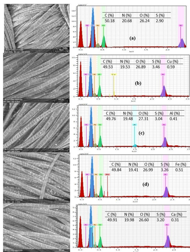
Fig. 6. EDX spectra of wool fabrics treated with 5% owf SL using no mordant (a) and Cu (b), Al (c), Fe (d), and Ca (e) mordanting agents.
