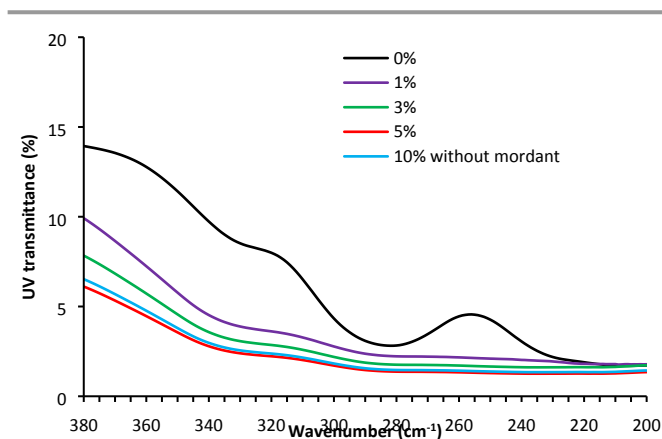
Fig. 7. Effect of SL concentration on the UV transmission through the wool fabric samples treated with SL using Cu as a mordanting agent.
