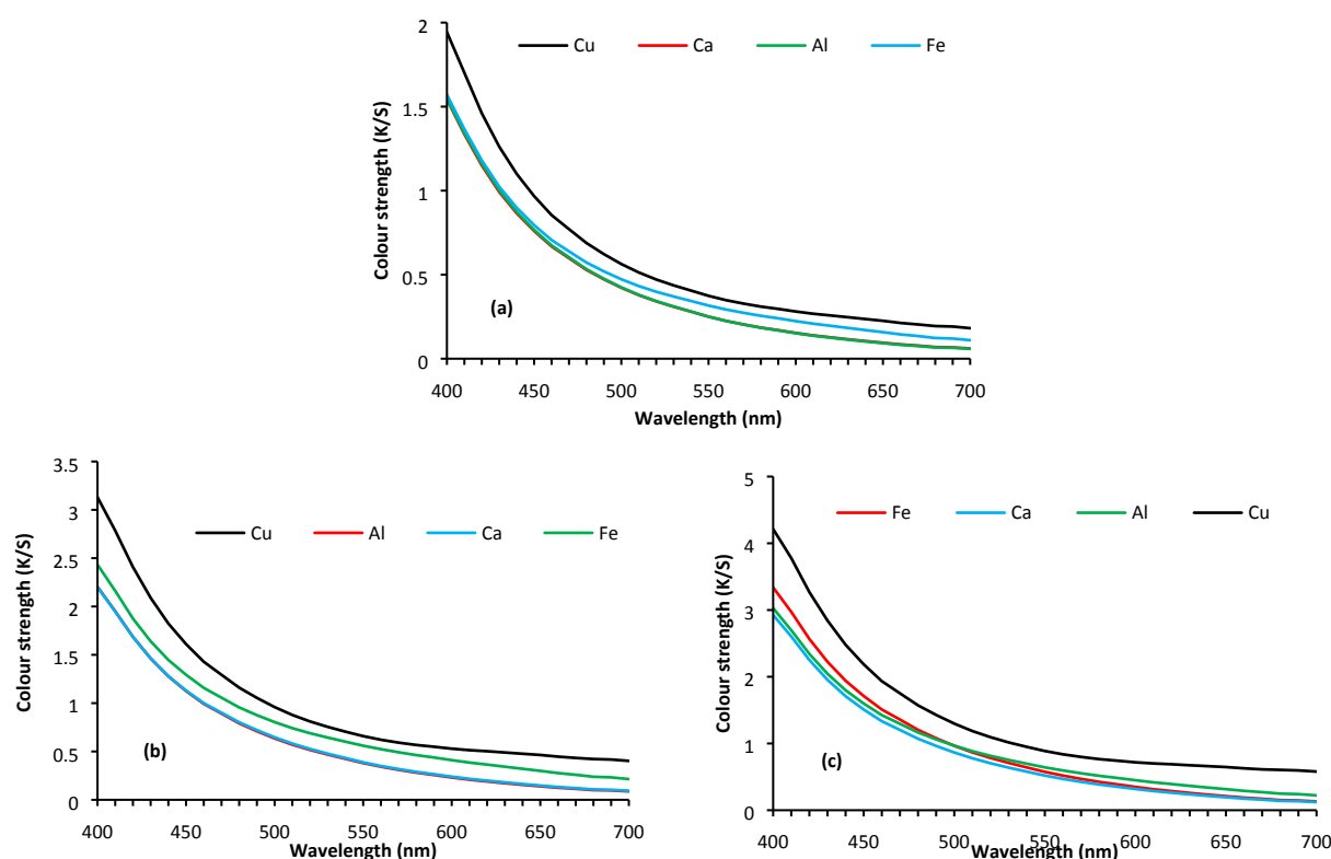
Fig. 3. Colour strength wool fabric dyed with 1(a), 3 (b), and 5% (c) SL using various metals at 25% ows.
