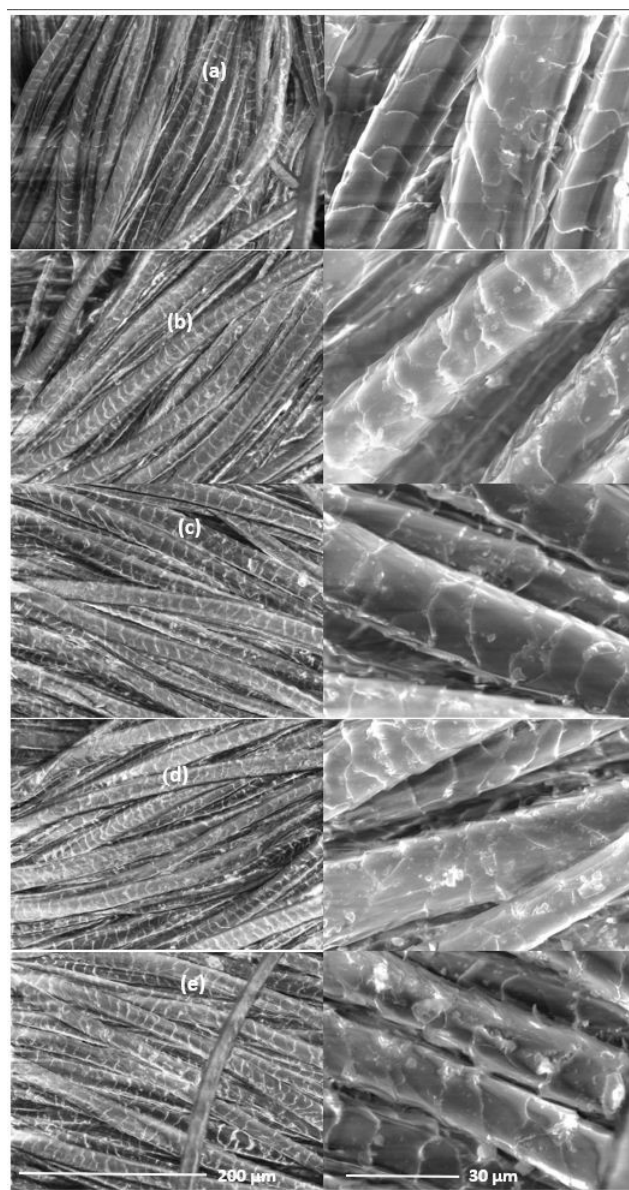
Fig. 8. SEM micrographs of surfaces of control wool fabric (a), and also wool fabric samples treated with 5% owf SL using 25% owf Al (b), Ca (c), Cu (d), and Fe (e).
