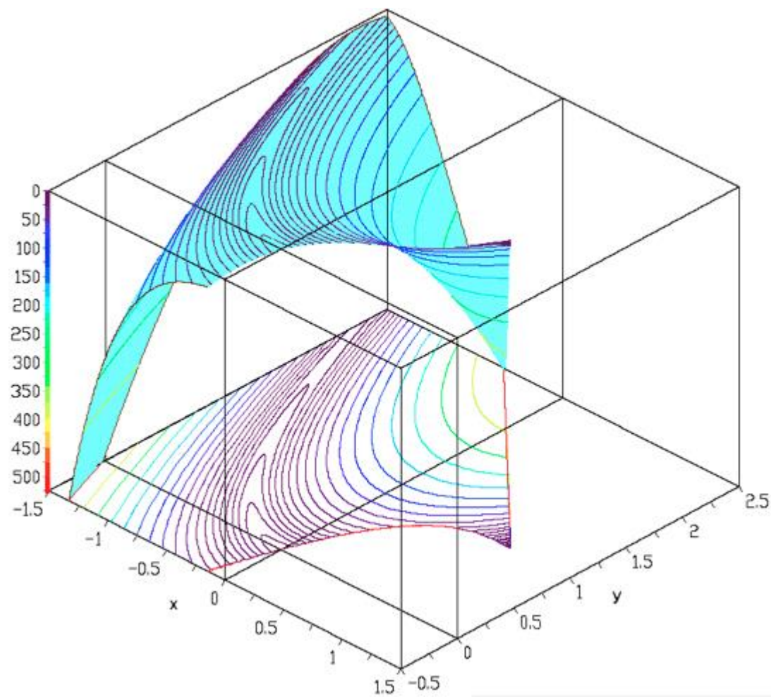
Figure 6: The Rosenbrock function used to test constrained optimization.
