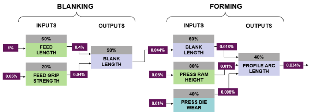
Figure 5: Complete FDD
