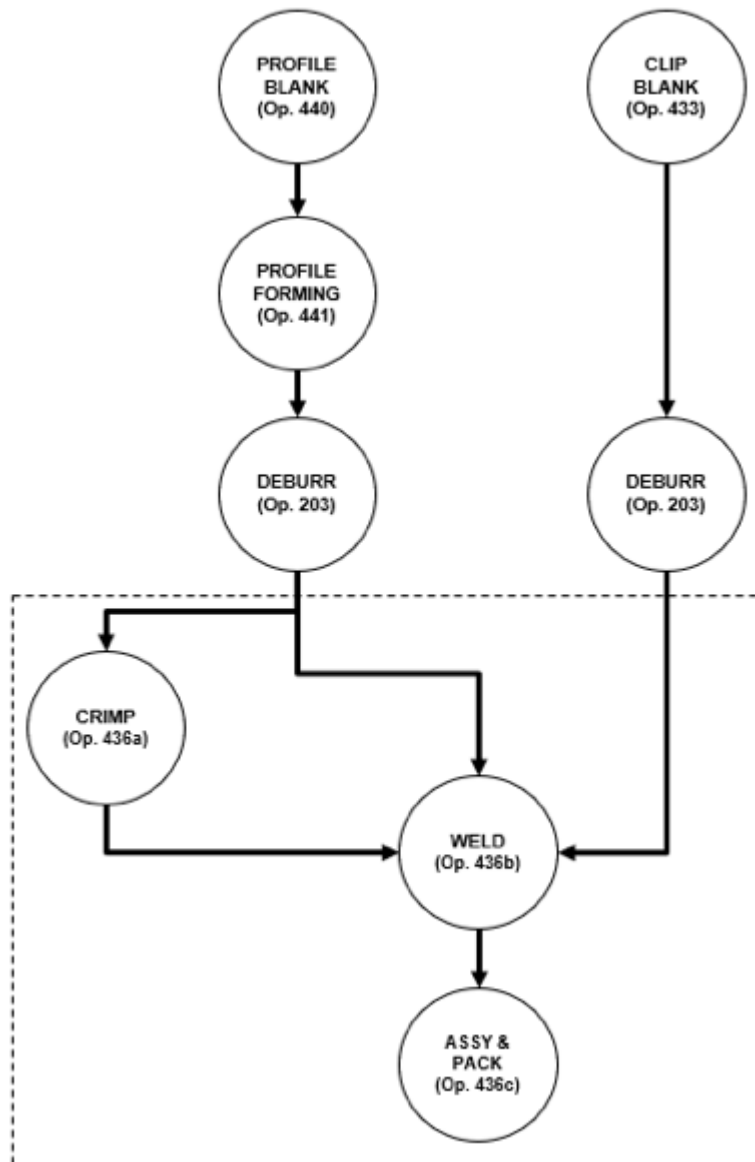
Figure 7: The VPP 096 Clamps processing flow diagram
