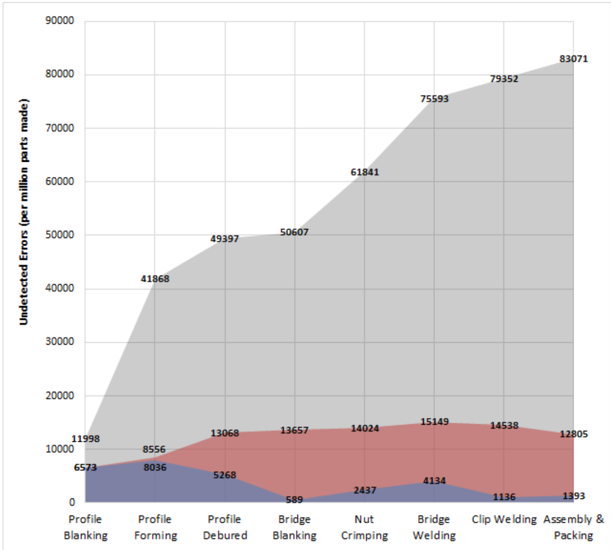
Figure 8: Errors present at each stage of production of a VPP clamp with an overhead clip. In blue: Undetected errors produced by each process. In red: Cumulative undetected errors after each process. In grey: Total undetected errors + detected errors after each process.
