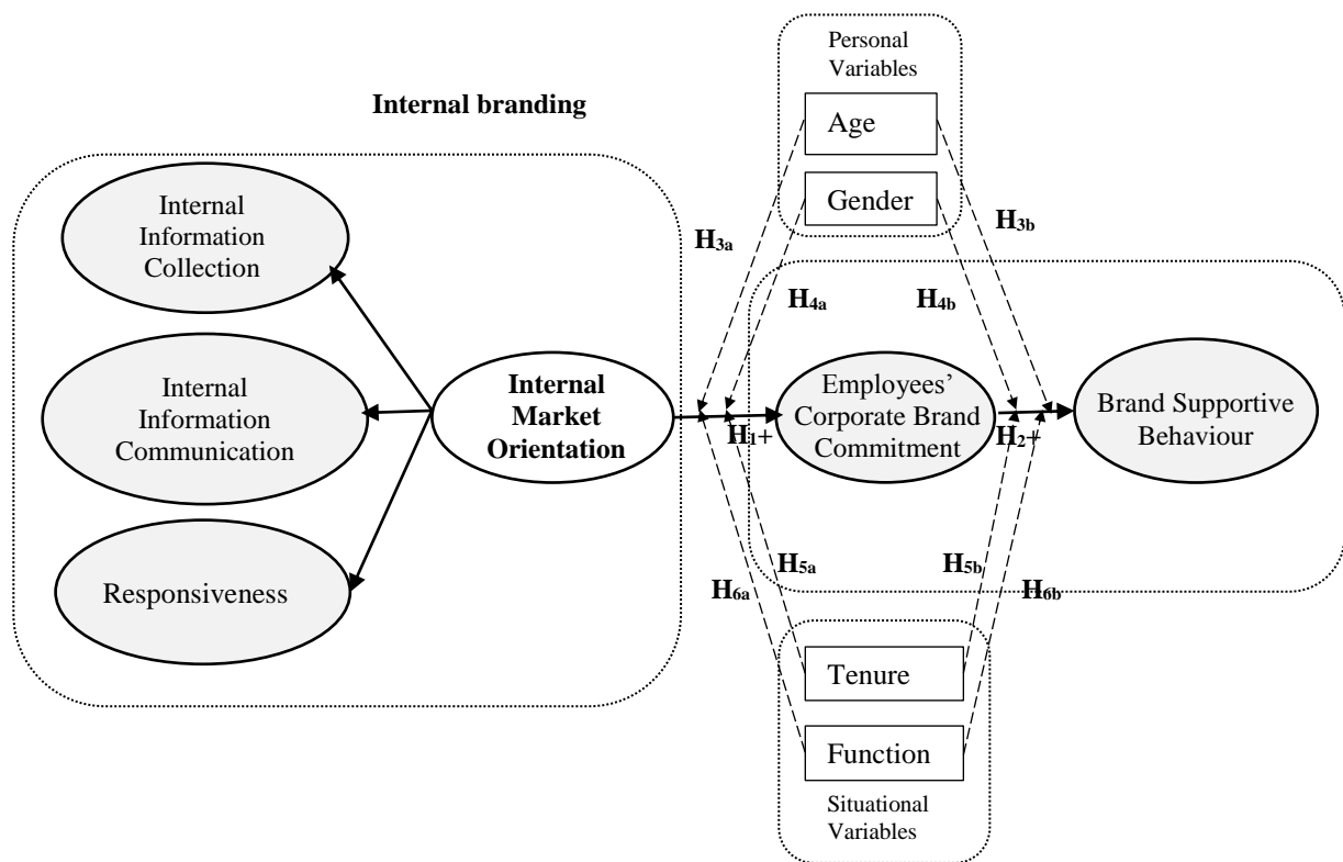
Figure 1: Conceptual Framework
