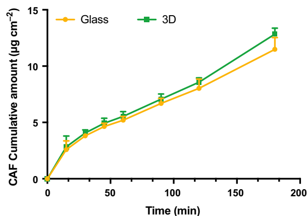
Figure 5 Amount of CAF permeation from initial dose per cm 2 of PDMS membrane at 0, 15, 30, 45, 60, 90, 120 and 180 min using glass and 3D-printed Franz type diffusion cells ( n = 4 , mean \pm SD).
