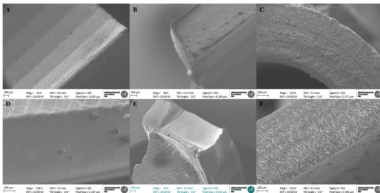
Figure 4 SEM micrographs of AM Franz type diffusion cell from pre-compatibility study: (A) inner wall receptor compartment, (B) y-edge overview receptor compartment, (C) full section collection arm; and after 72 h post-compatibility study: (D) cut inner wall receptor compartment, (E) overview wall receptor compartment, (F) overview of edge cut from collection arm.
